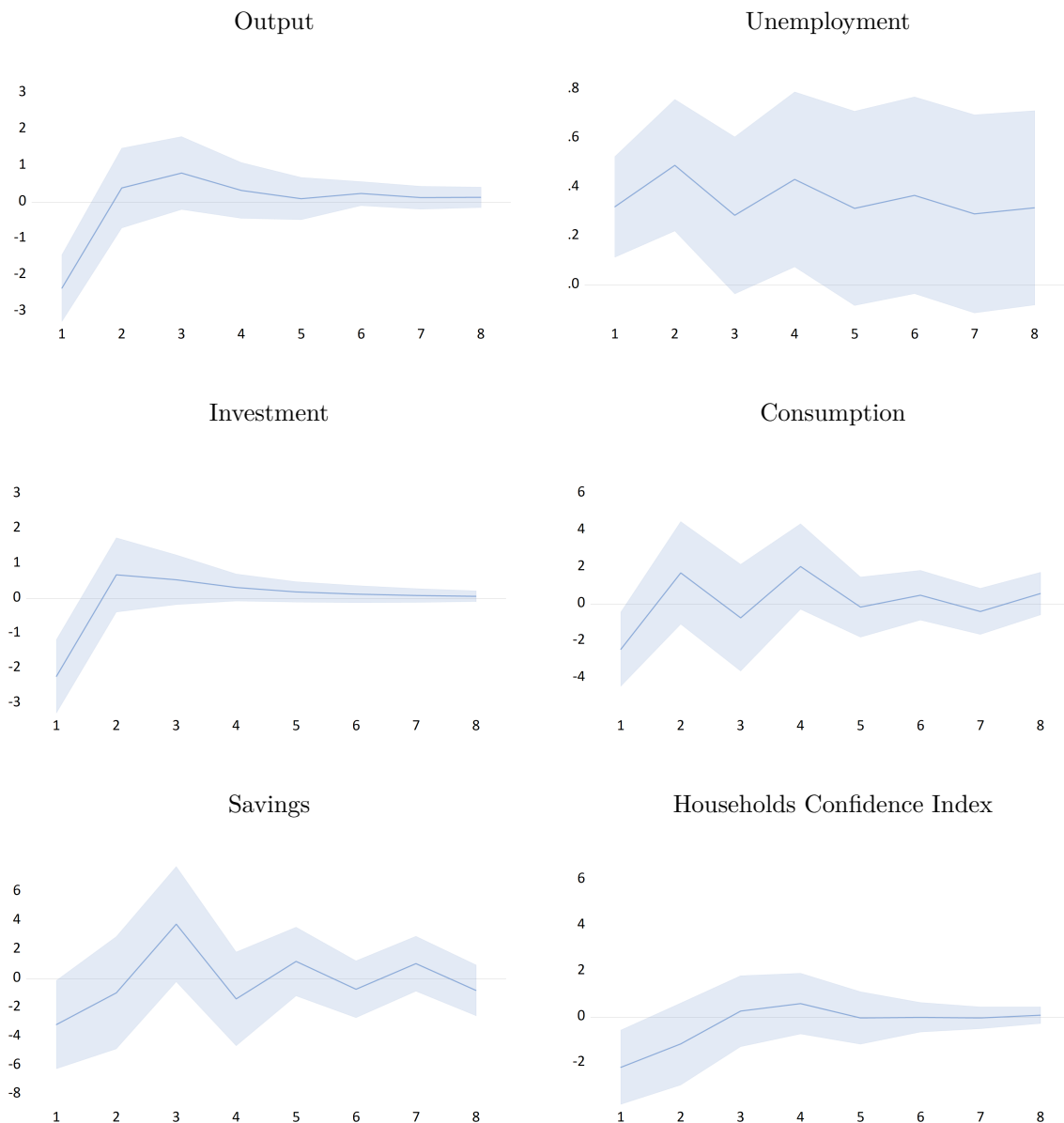
Figure 4 Impulse responses to one-standard deviation EPU shocks
